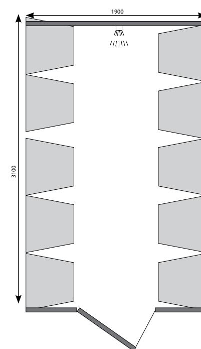
Model 10BC 10 bathers 3100 x 1900 x 2250mm
