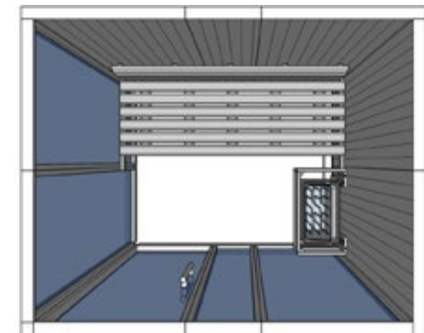
V2025 2 bathers 1675 x 1368 x 1950mm
