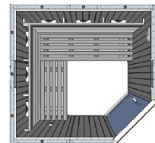
IR4030 8 bathers 2480 x 1960 x 1950mm
