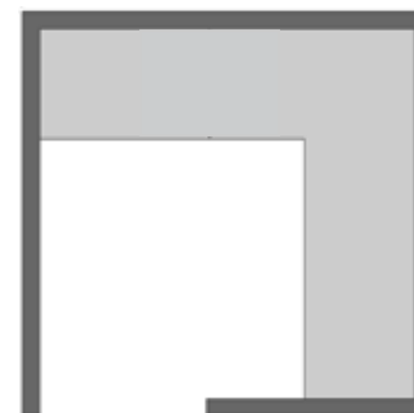
Model 3 4 bathers 1966mm x 1946mm x 2400mm
