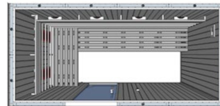
IR2040 4 bathers 2580 x 1250 x 1950mm
