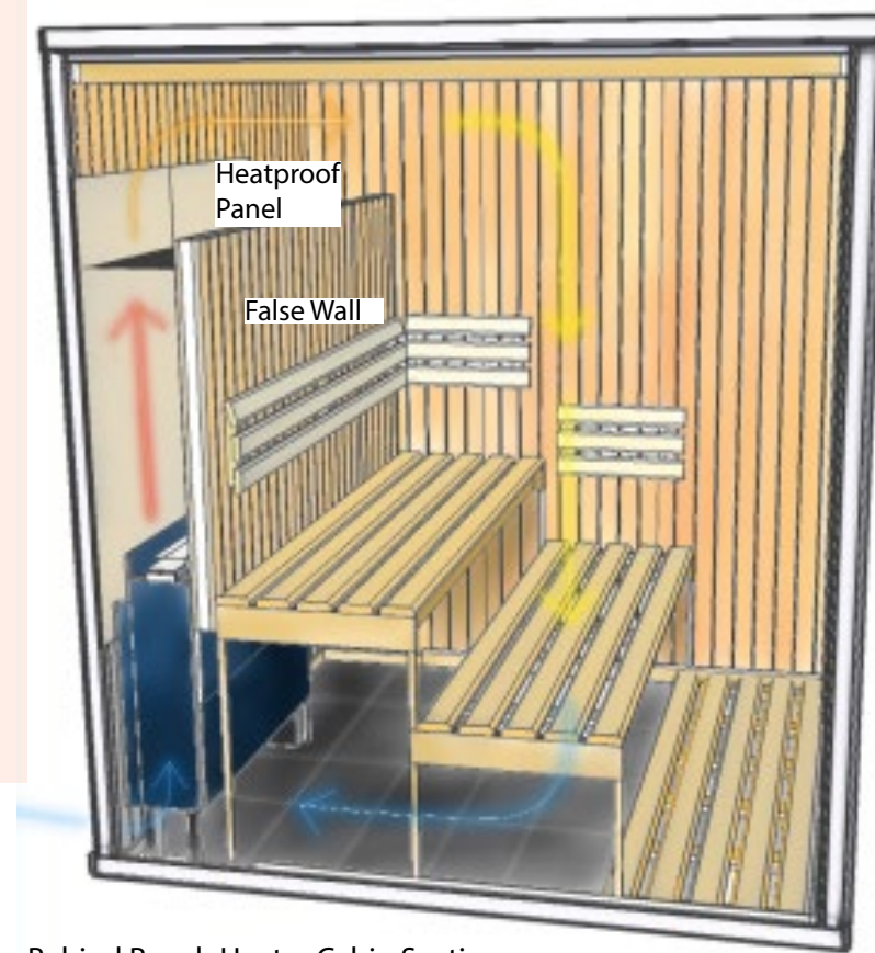
Behind Bench Heater Cabin Section
