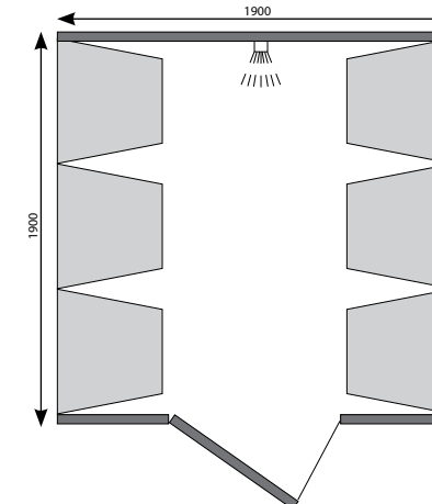
Model 6B with door positioned to the right
