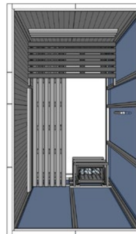
V2035 4 bathers 2290 x 1368 x 1950mm
