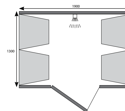
Model 4B 4 bathers 1900 x 1300 x 2250mm
