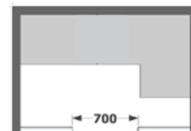
Model 2 C 2 bathers 1966 mm x 1346mm x 2400mm
