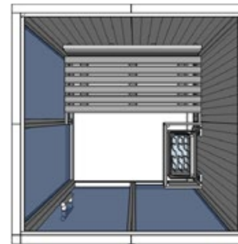
V2020 1-2 bathers 1368 x 1368 x 1950mm
