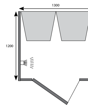
Model 2B 2 bathers 1300 x 1200 x 2250mm
