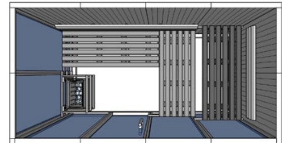
V2040 5 bathers 2600 x 1368 x 1950mm
